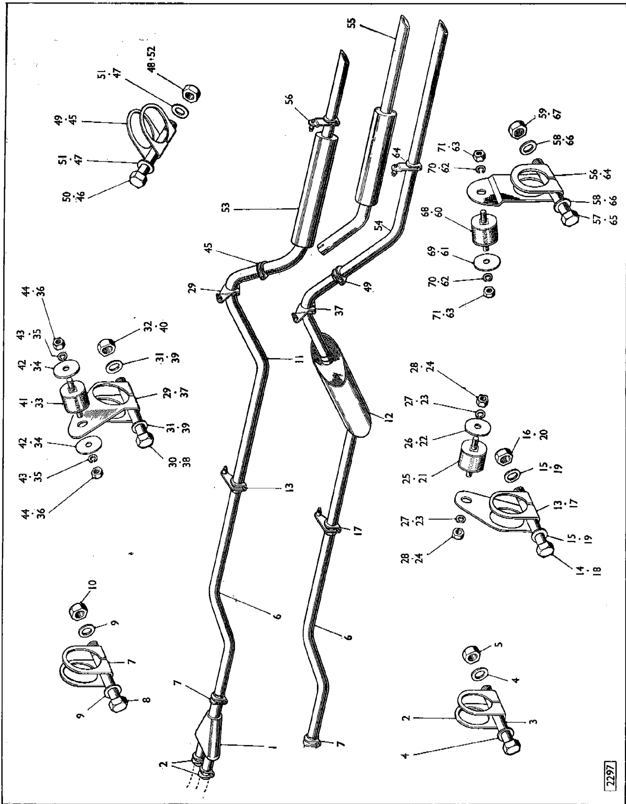
SECTION V
