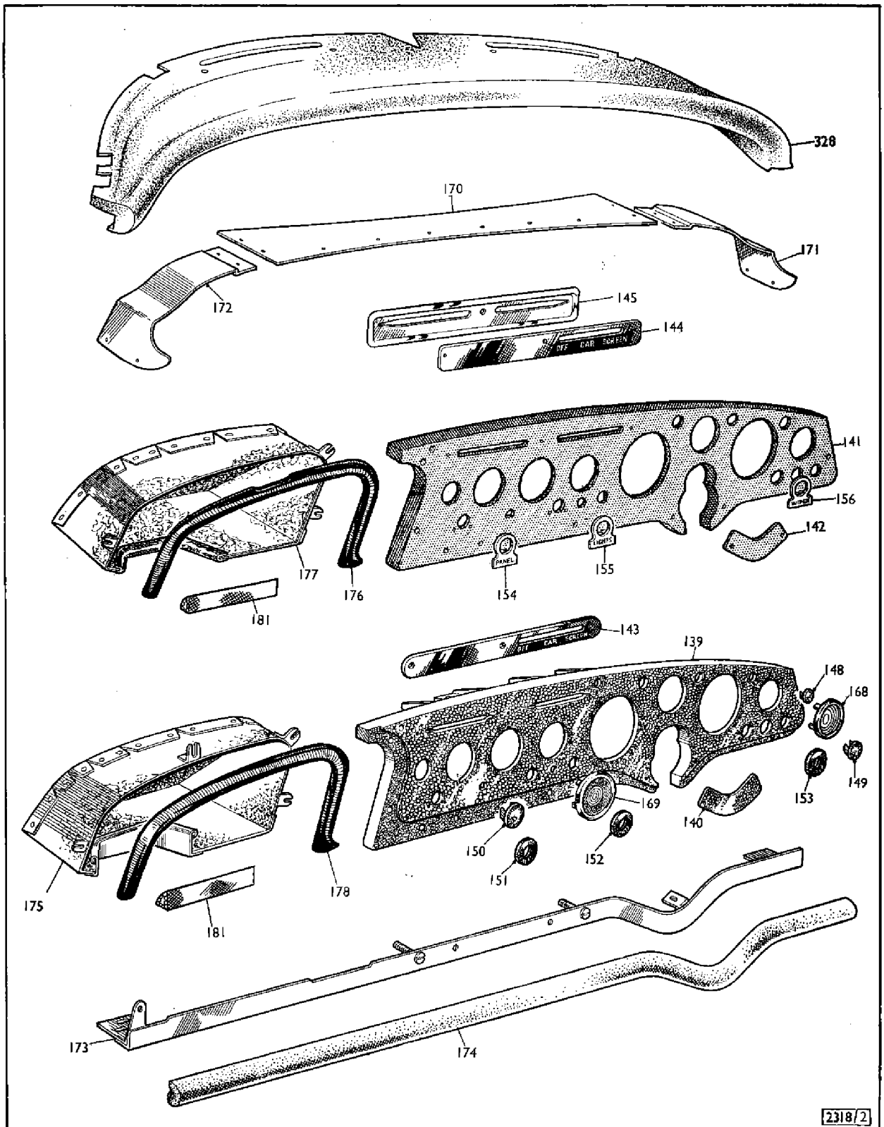
PLATE C — SECTION YX
