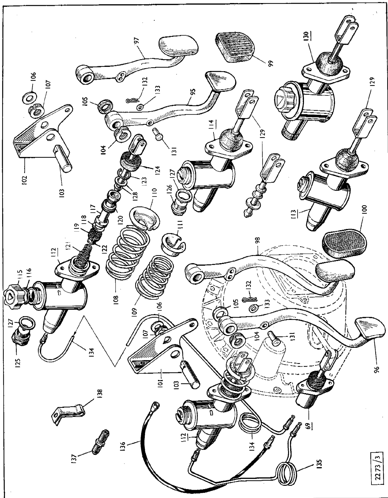
PLATE C – SECTION F
