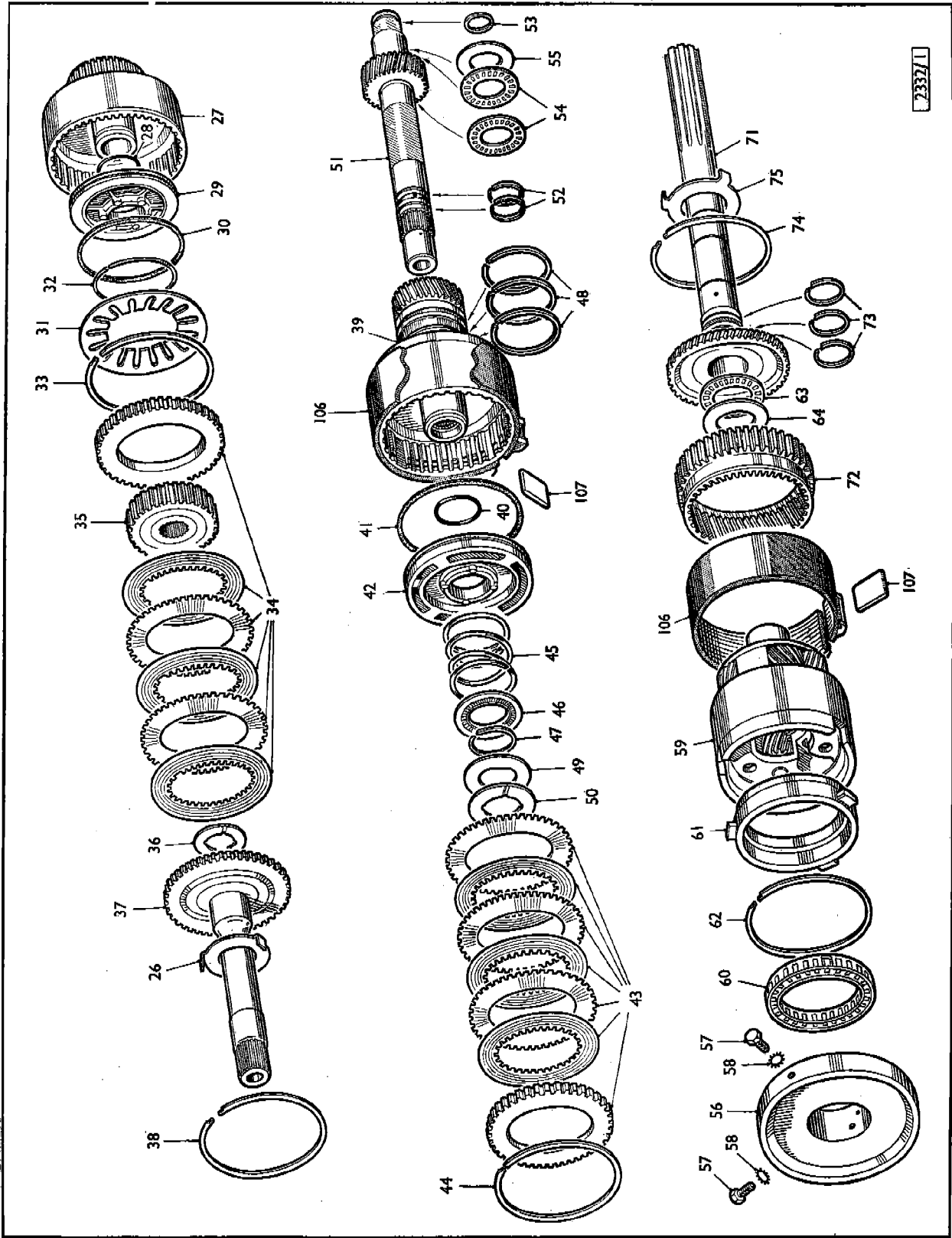
PLATE C — SECTION H
