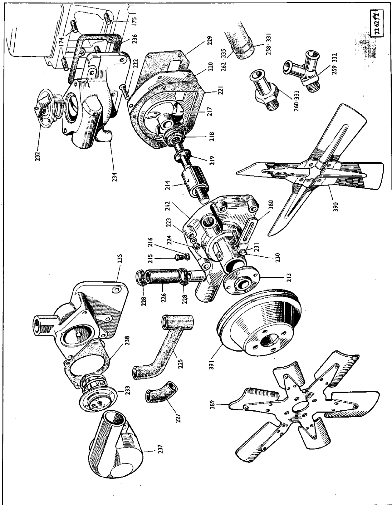
PLATE C — SECTION A
