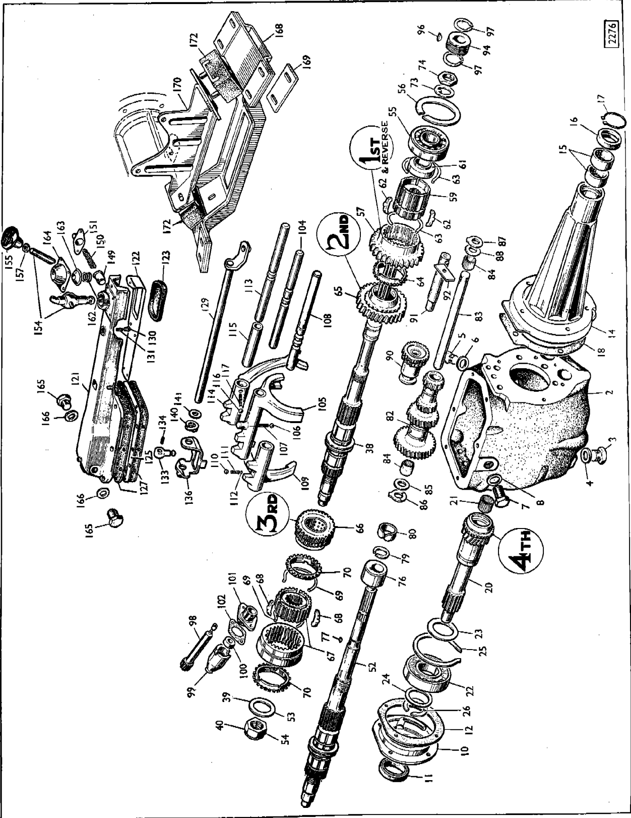
PLATE C — SECTION G
