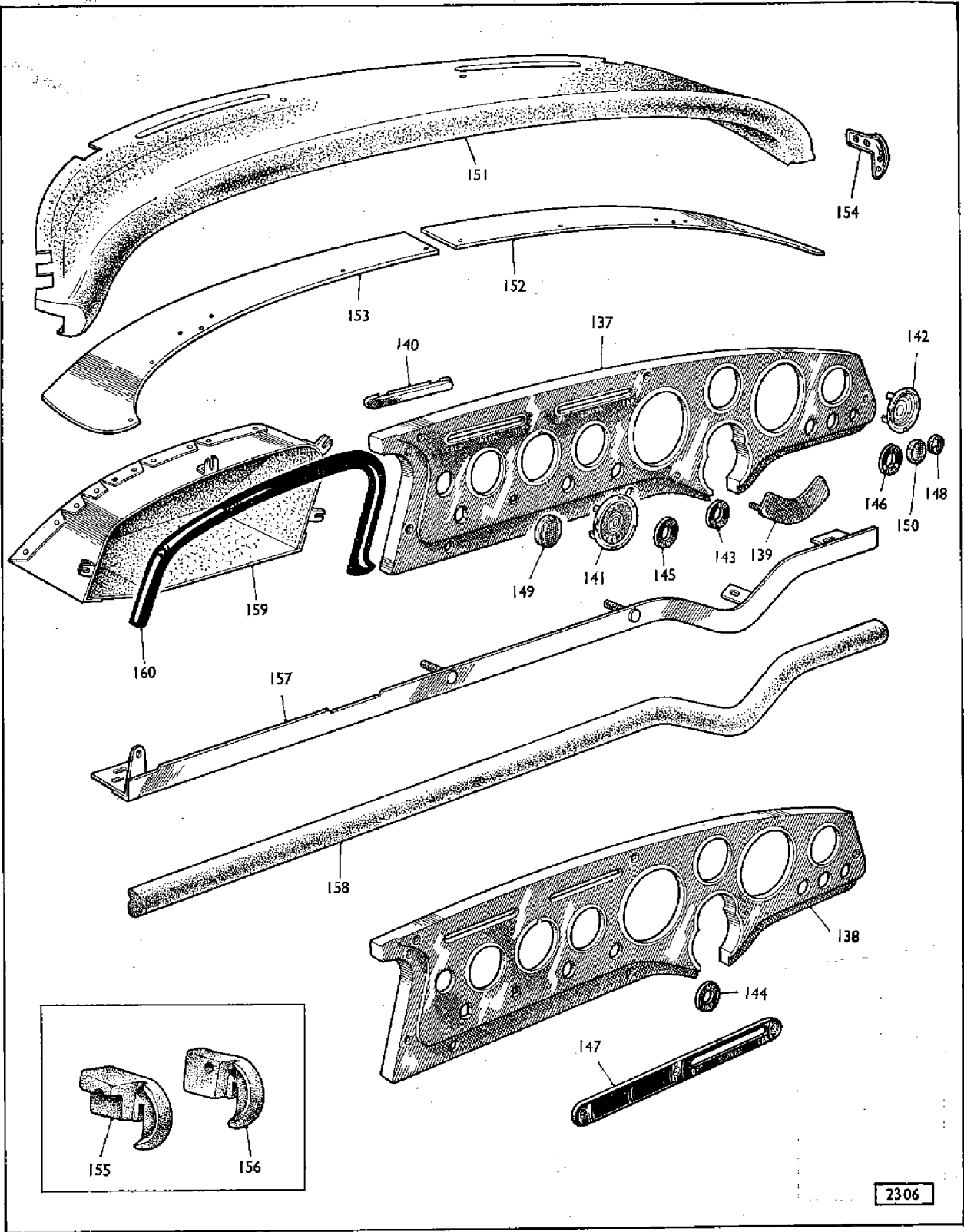
PLATE C — SECTION YV
