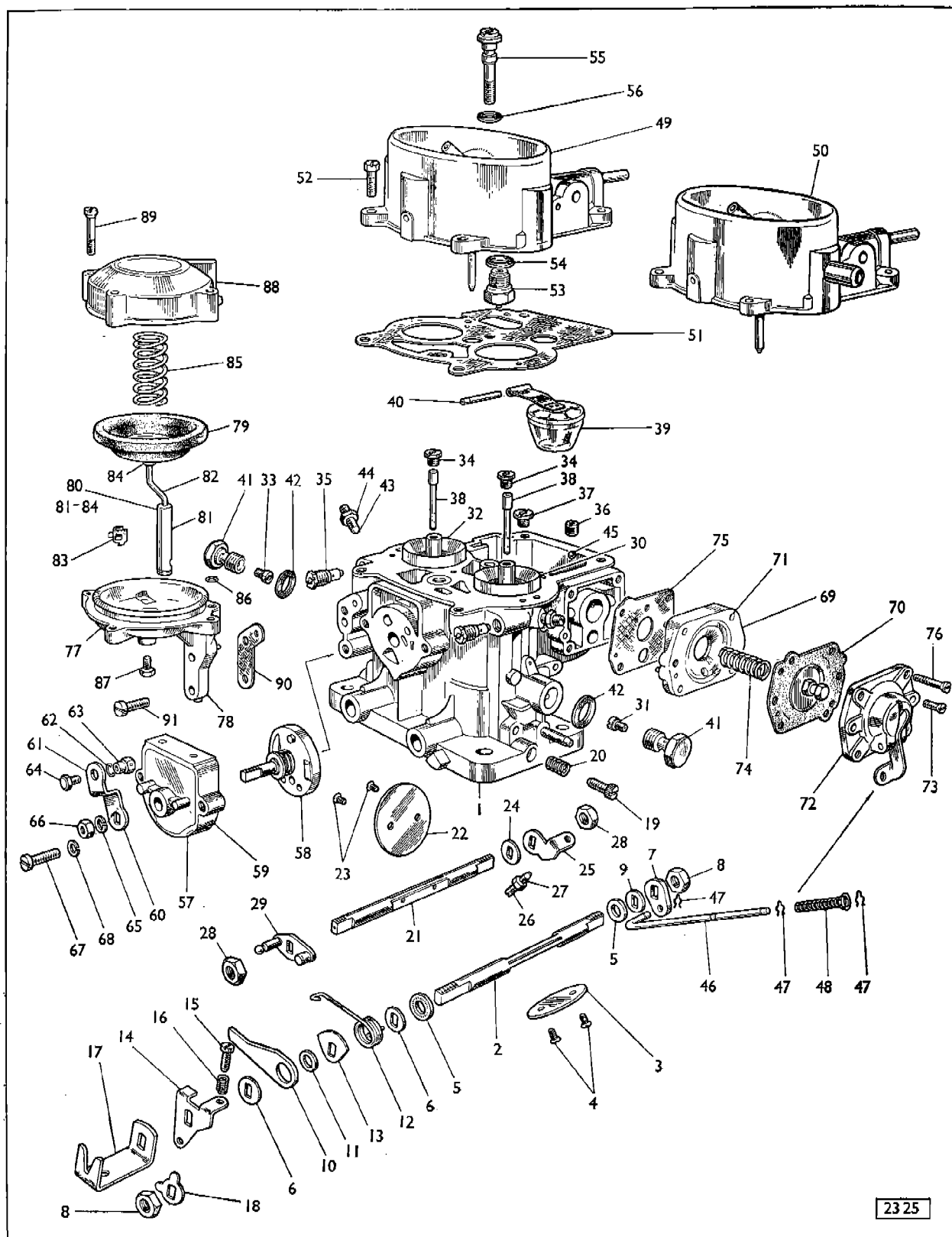
SECTION CB
