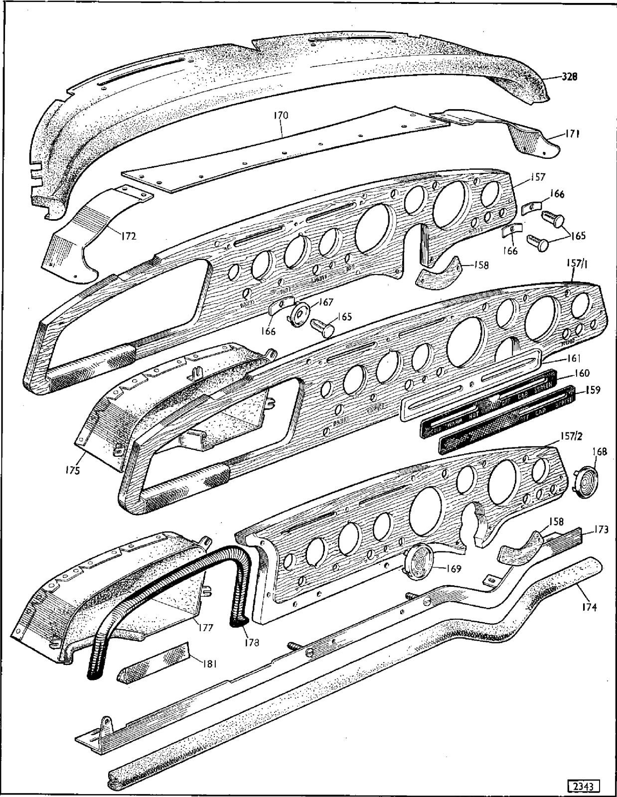
PLATE CA—SECTION YX
