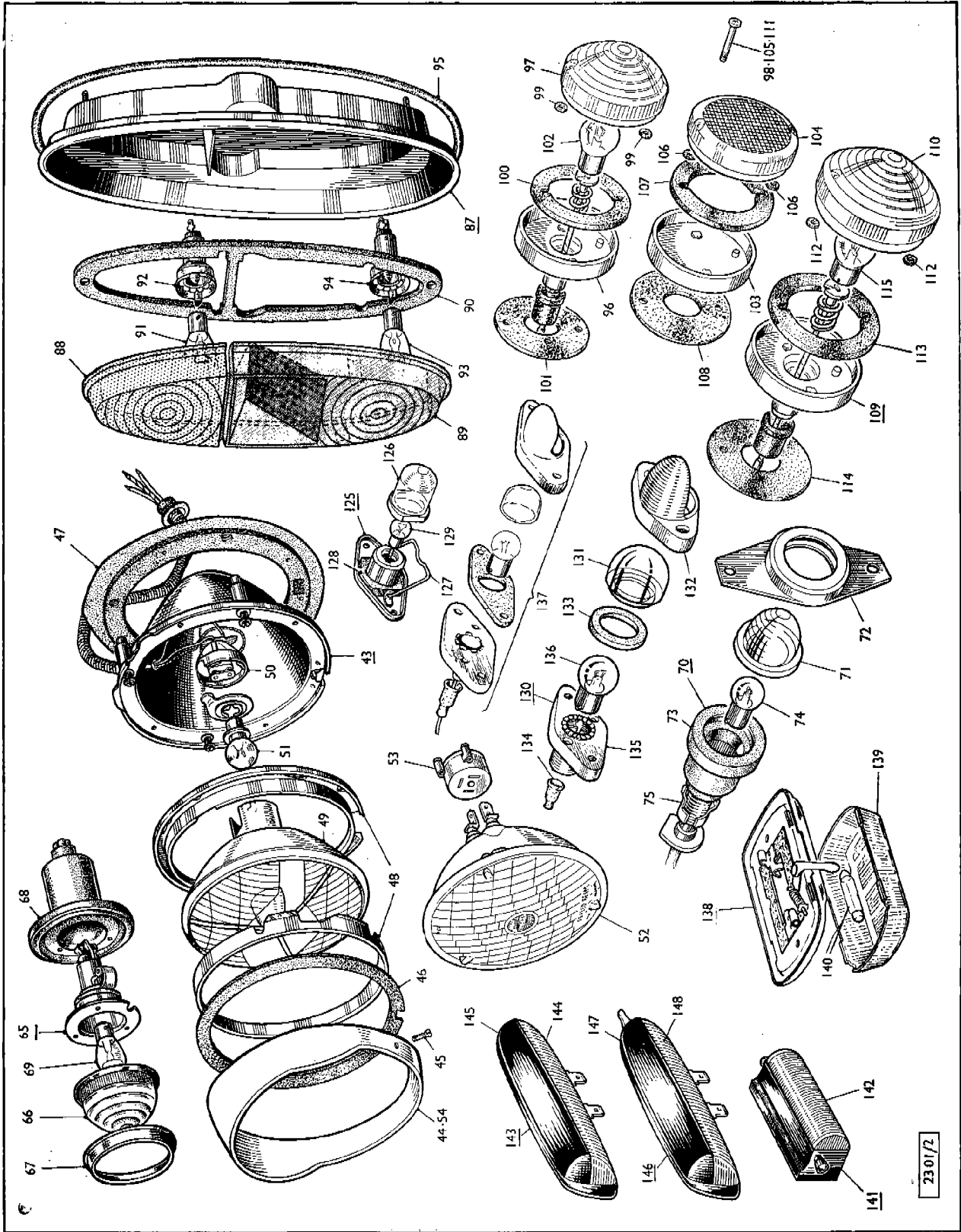
PLATE C — SECTION W
