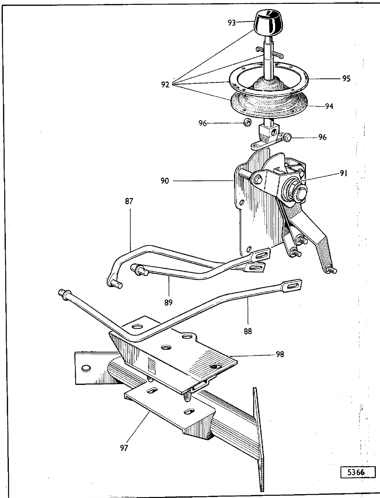
PLATE B — SECTION GF
